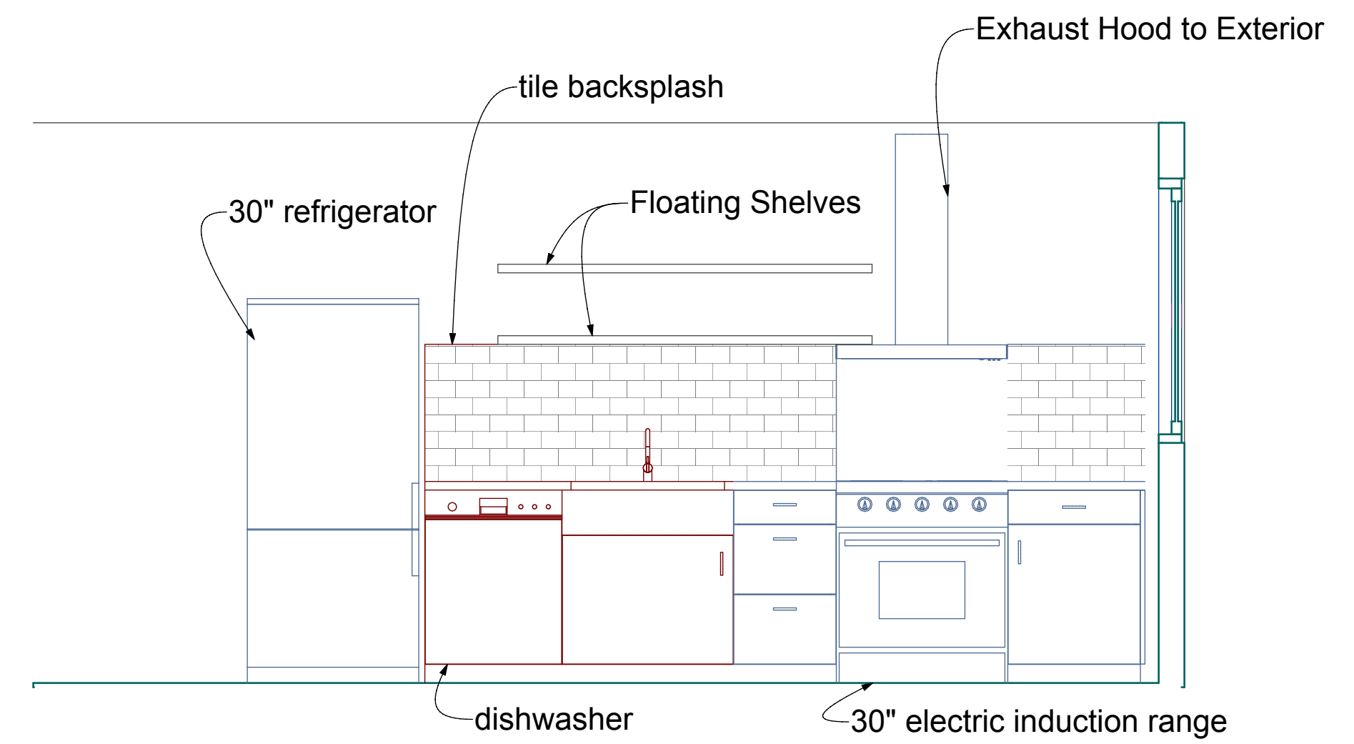
1 Kitchen Elevation SCALE: 1/2" = 1'-0"
