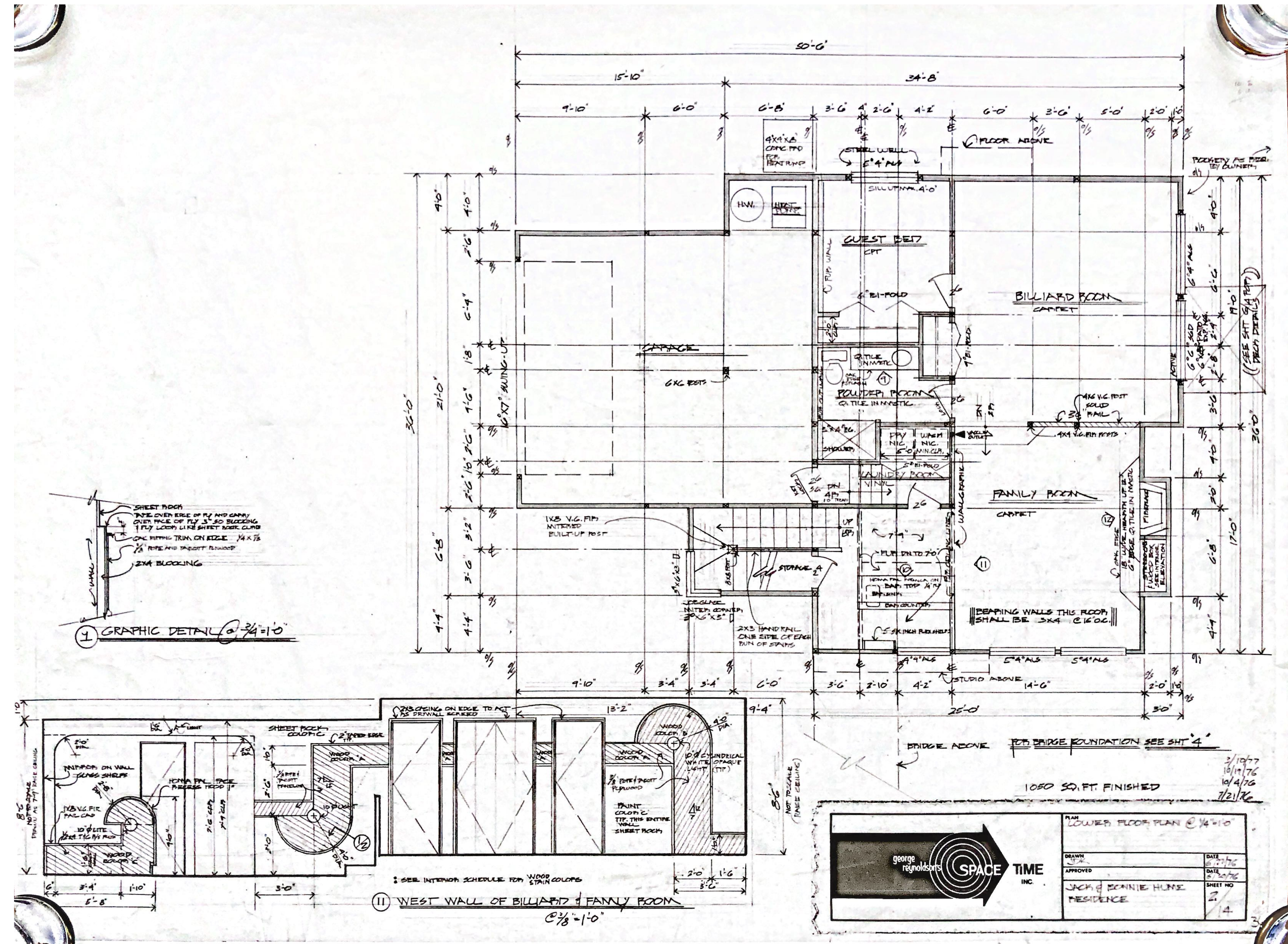
1 Scan of Space Time Plans - Lower Floor A7 SCALE: 1/4" = 1'-0"
