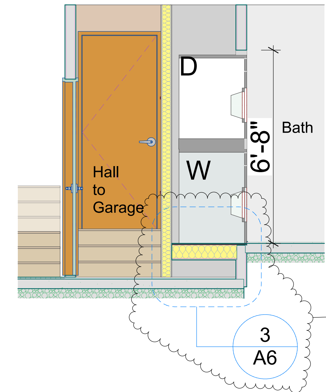
2 Section at Washers/Dryers (1) SCALE: 1/2" = 1'-0"
